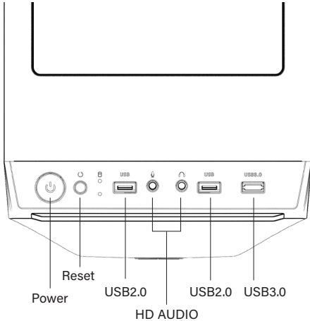
case AzaliaHD Audio connector
